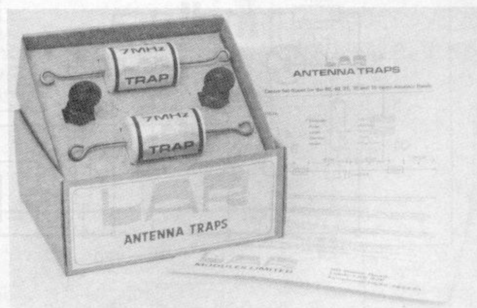
This attractively boxed pair of 7 MHz weather-proof traps (500-watt rating) comes from LAR Modules Ltd., 60 Green Road, Leeds LS6 4JP. Included in the package are a pair of lightweight end insulators and full instructions for making a 5-band trap dipole. The price inclusive of VAT and post/packing is £14.25.
