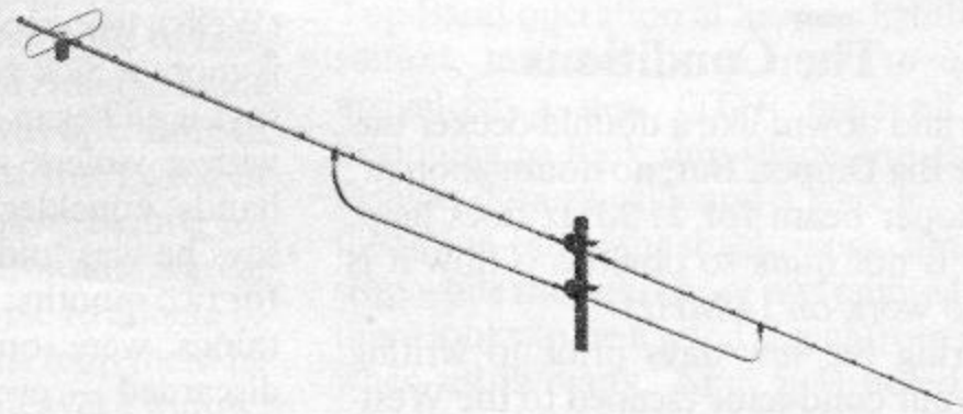
Above, a 23-element DL6WU long-yagi for 432 MHz with 17.9dBi gain. Below, a 70cm. antenna system using four 23-element DL6WU yagis stacked vertically giving approximately 23dBi gain, vertical polarisation being provided by a pair of 16-element DL6WU's giving about 19dBi. These antennas, which are made in Germany by H.A.G., are obtainable through the sole UK agent, muTek Limited , Bradworthy, Holsworthy, Devon EX22 7TU (tel: 040924-543/8), who should be contacted for full details, specifications and prices.
