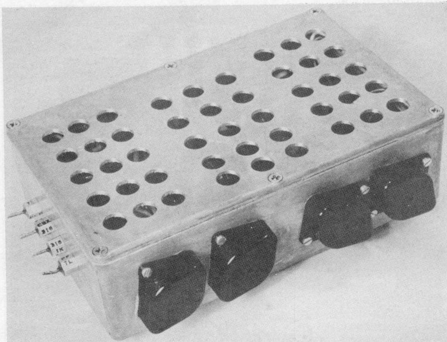
A 300V variant, Here the transistors are mounted on the box itself, and must be insulated with TO3 transistor covers as shown. Note the extra ventilation holes in the lid, in conjunction with a pair of similar holes in the base; the box is held off-chassis with tapped spacers, which permits cooling airflow.
