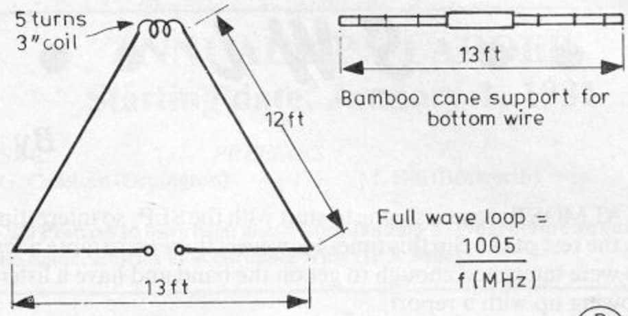
Fig. 2 DELTA FOR 21 MHz
