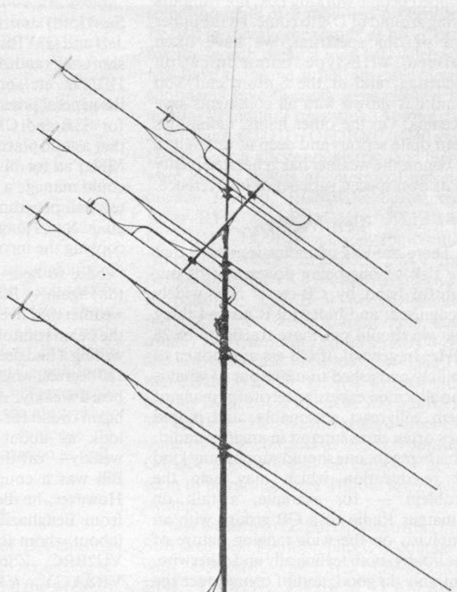
Above, a 23-element DL6WU long-yagi for 432 MHz with 17.9dBi gain. Below, a 70cm. antenna system using four 23-element DL6WU yagis stacked vertically giving approximately 23dBi gain, vertical polarisation being provided by a pair of 16-element DL6WU's giving about 19dBi. These antennas, which are made in Germany by H.A.G., are obtainable through the sole UK agent, muTek Limited , Bradworthy, Holsworthy, Devon EX22 7TU (tel: 040924-543/8), who should be contacted for full details, specifications and prices.
